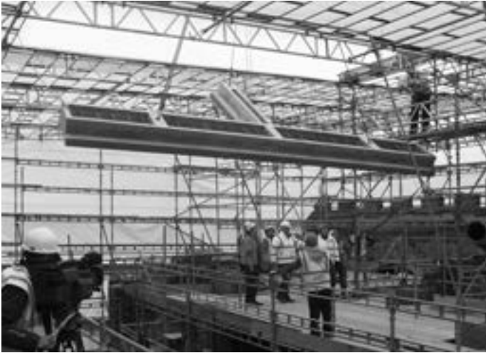
Astley Castle, lowering the hollow concrete 'T' lintel into place
